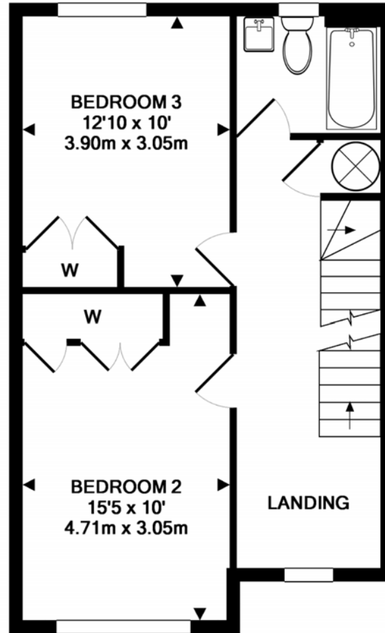
1ST FLOOR
